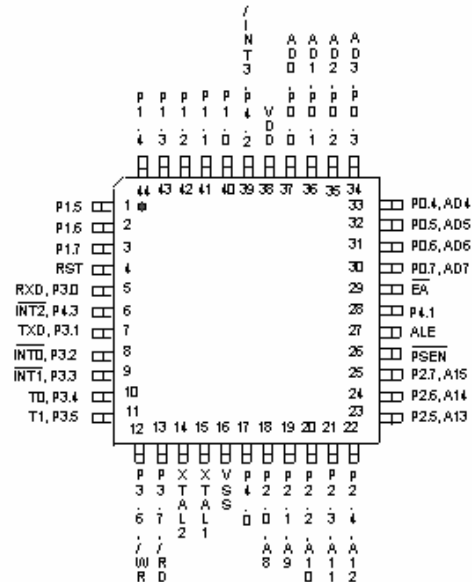
44-Pin QFP
