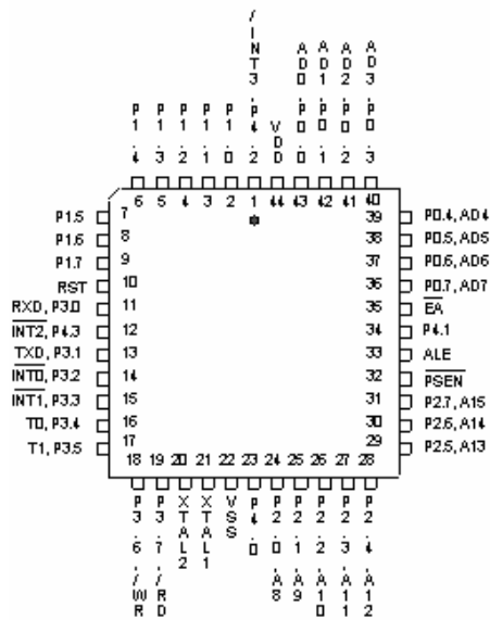
44-Pin PLCC
